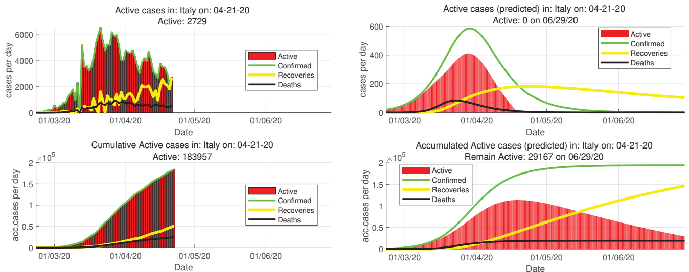
Fig. 26 Active cases reported and predicted from the SIR model without vital dynamics until the end of the first cycle of the activity of coronavirus for Italy
