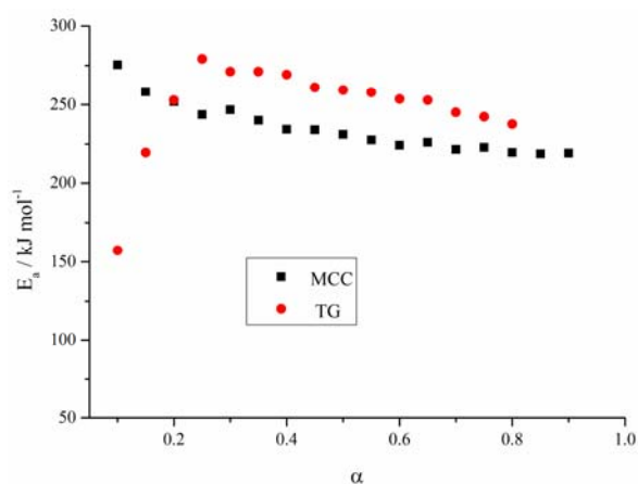
Fig. 11 Variation of E_a from MCC and TG for grey XPS
